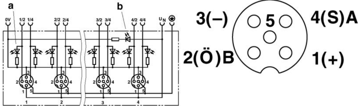
Schematic diagram
